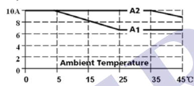
Output Current
