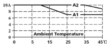
Output Current
