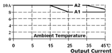
Output Current
