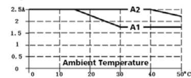
Output Current
