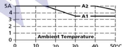
Output Current
