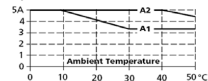
Output Current
