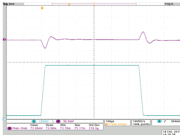
Transient Response
