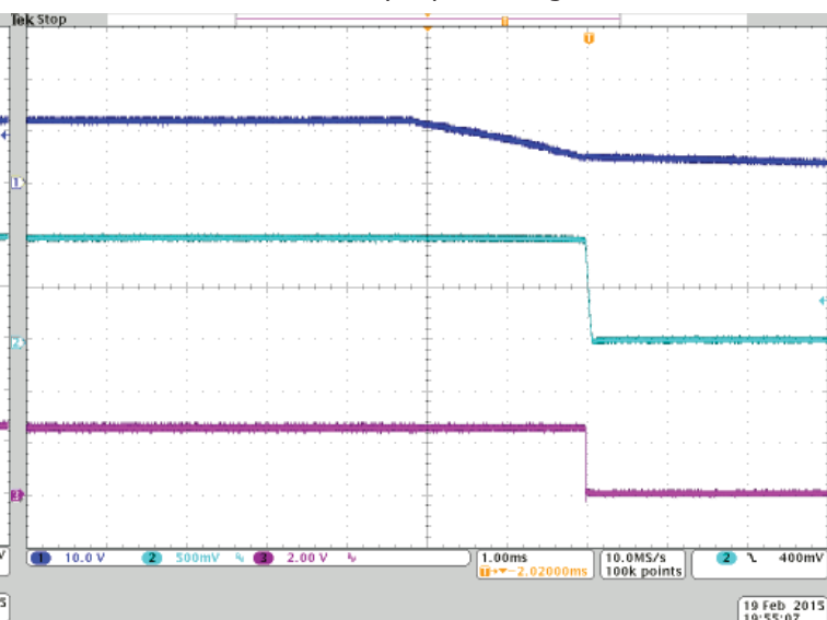
Disable by CTRL pin
