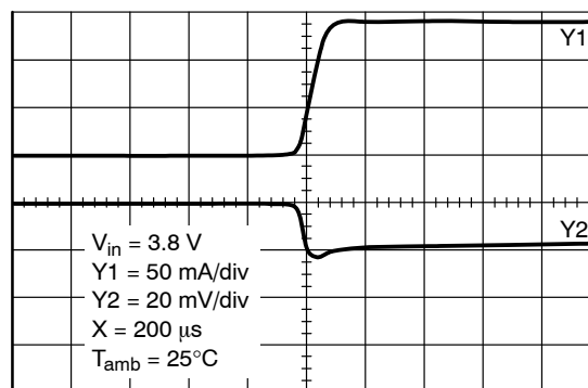
Figure 25. I_{Slope} = 2.0 \text{ mA}/\mu\text{s} (Large Scale) I_{out} = 3.0 \text{ mA to } 150 \text{ mA}
