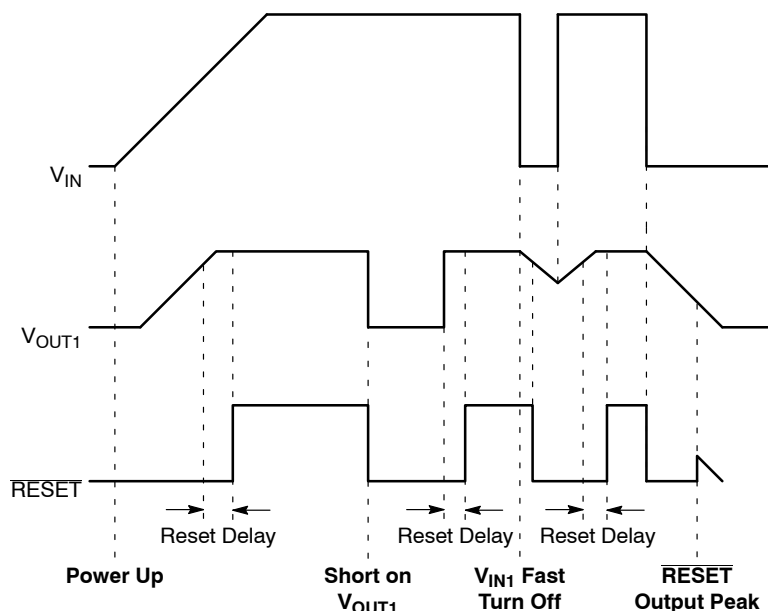
Figure 41. Dual Drive \overline{\text{RESET}} Valid
