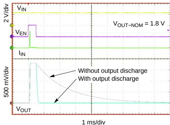
Figure 25. Turn-ON/OFF – EN Driven
