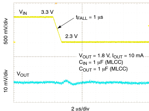
Figure 37. Line Transient Response – I_{OUT} = 10 \text{ mA}
