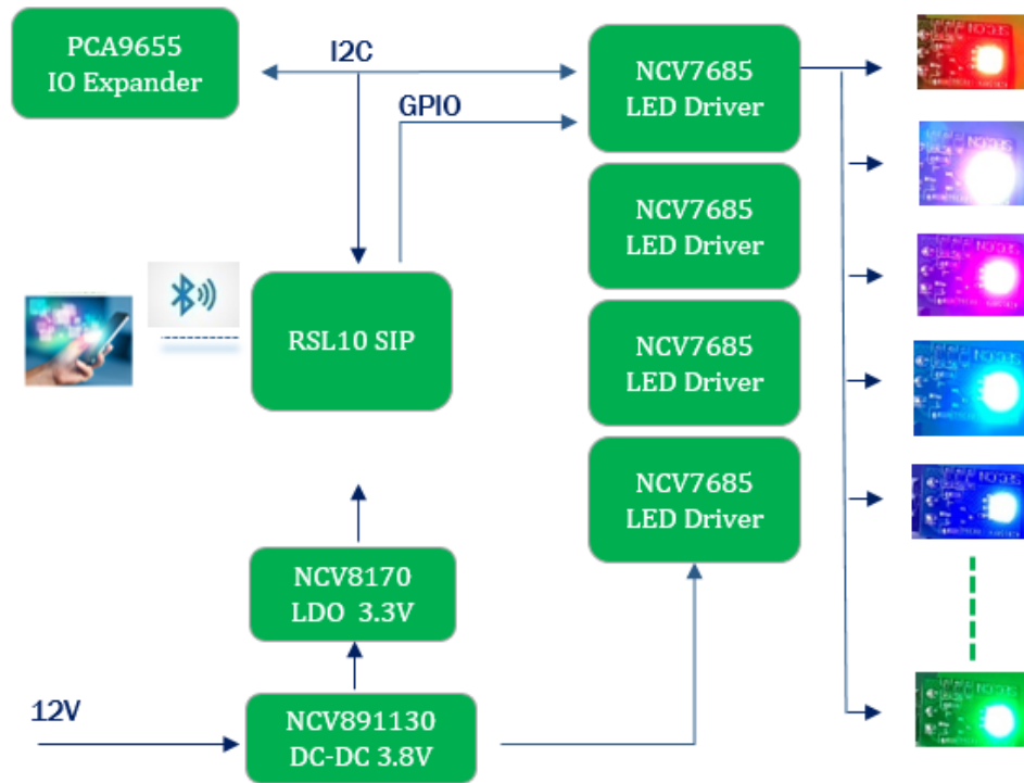
Figure 1. Board Architecture
