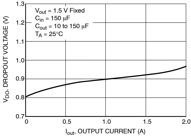
Figure 6. 1.5 V Dropout Voltage vs. Output Current
