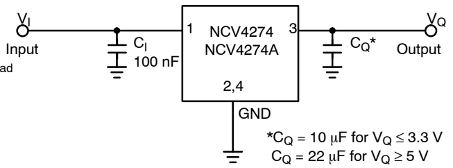
Figure 3. Application Circuit
