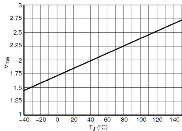
Figure 13. Thermal Warning Threshold in Function of Junction Temperature
