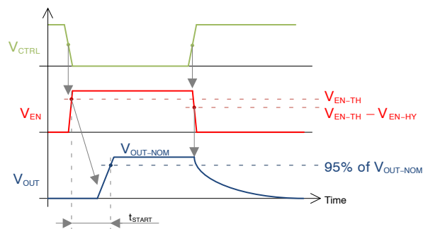
Figure 56. Startup Timing – EN Pin Controlled by Transistor
