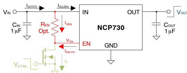
Figure 55. Circuit – EN Pin Controlled by Transistor
