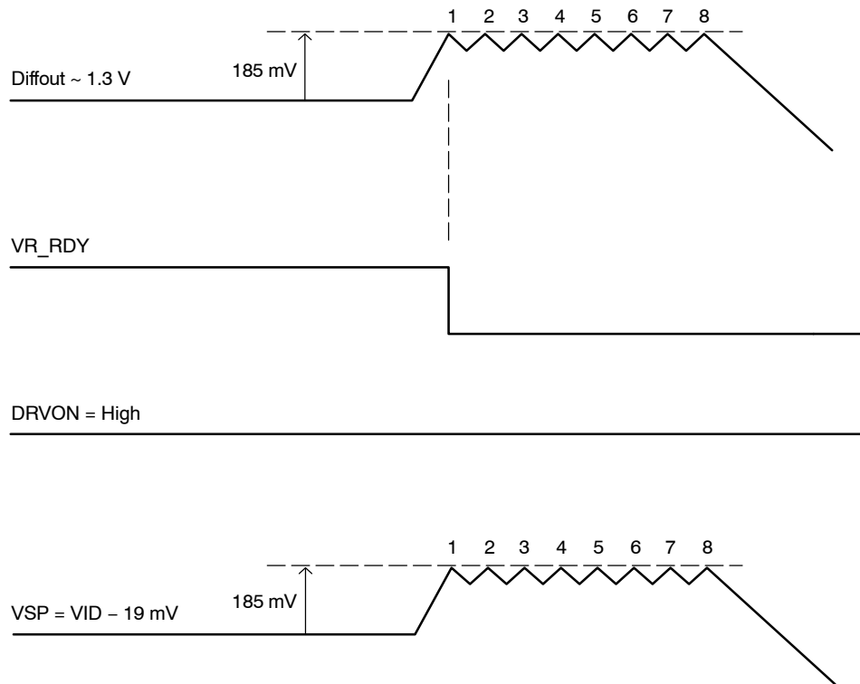
Figure 26. OVP Shutdown
