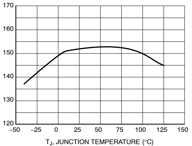
Figure 18. 2.55 V Reference Minimum Cathode Current for Regulation vs. Junction Temperature
