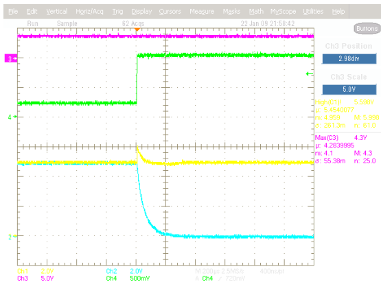
Figure 11. Disable time (200 \mu\text{s}/\text{div} , Ch1: V_{in} , Ch2: V_{out} , Ch3: \overline{FLAG} , Ch4: \overline{EN} )
