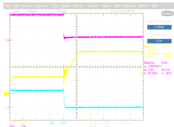
Figure 10. V_{in} rise to fault (100 \mu\text{s}/\text{div} , Ch1: V_{in} , Ch2: V_{out} , Ch3: \overline{FLAG} )
