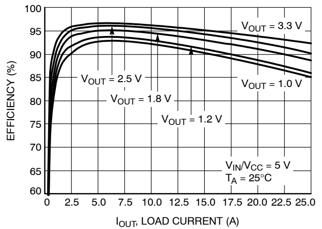
Figure 14. Efficiency vs. I_{out} ( V_{in} = 5\text{ V} )
