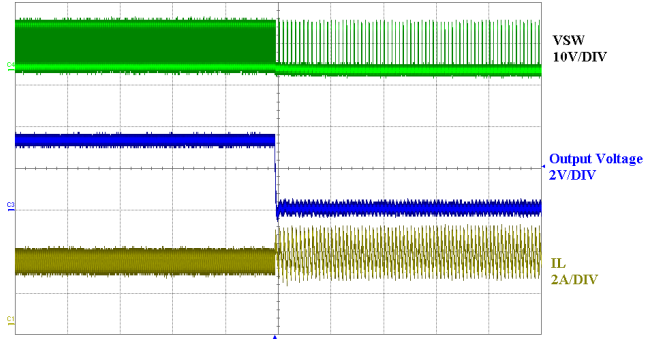
Figure 6. Short-Circuit Protection 200 \mu\text{s /DIV}
