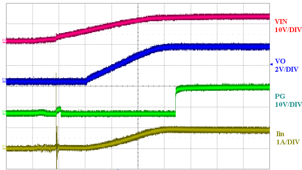
Figure 5. Start-Up into Full Load 1 \text{ms/DIV}
