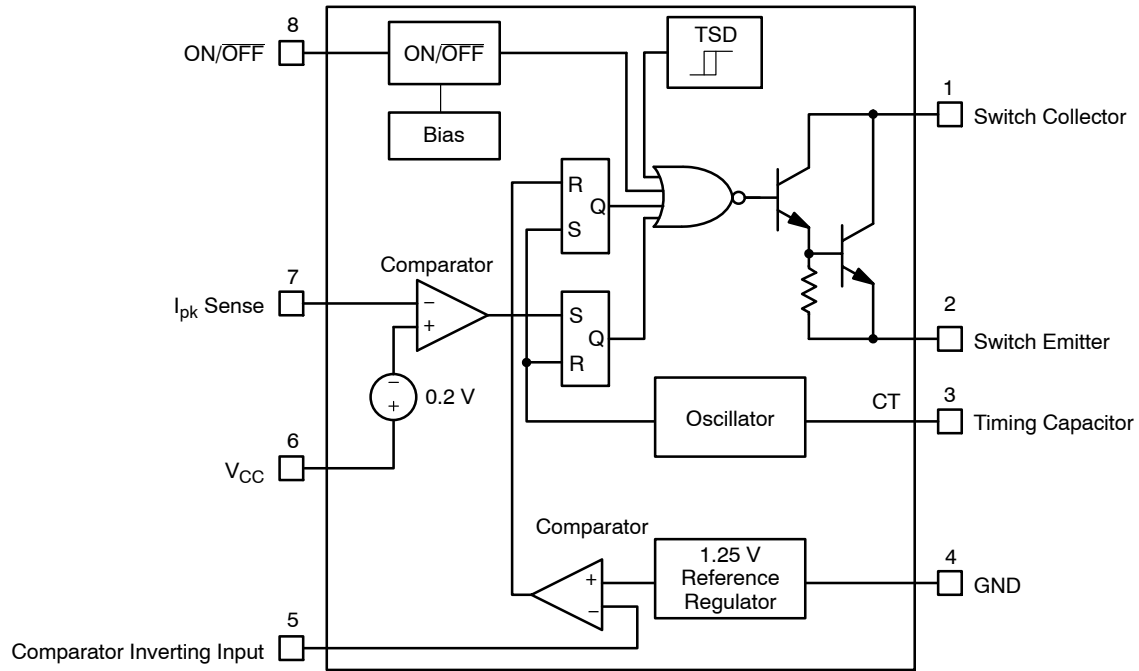
Figure 4. Block Diagram
