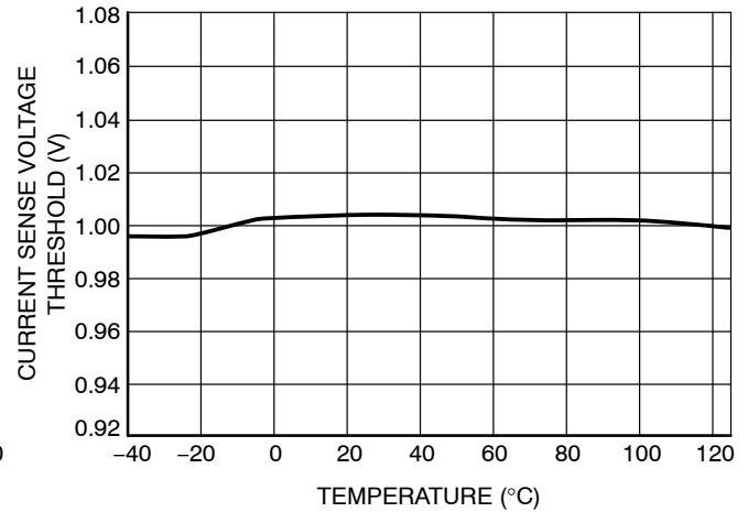
Figure 10. Current Sense Voltage Threshold vs. Junction Temperature
