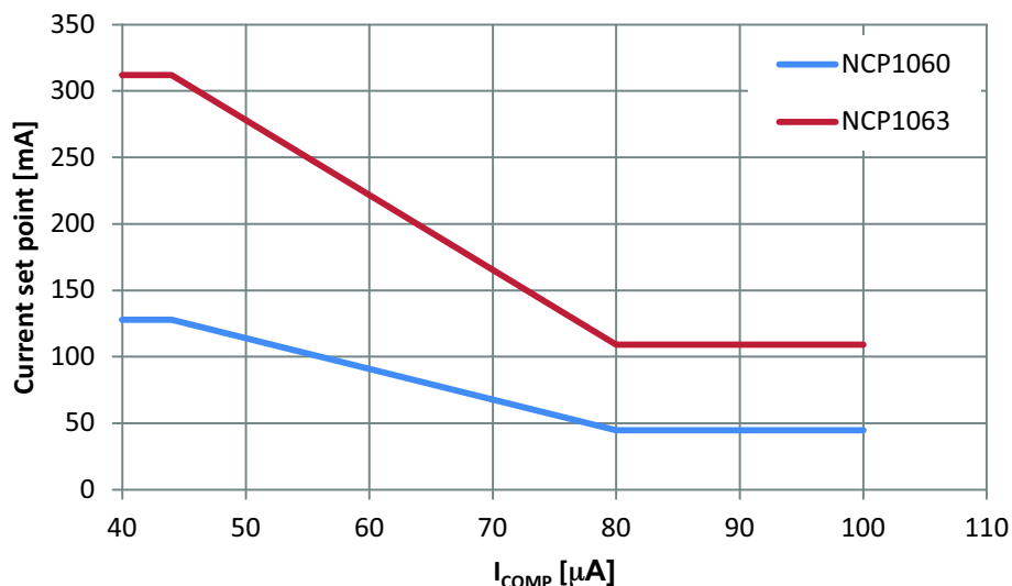
Figure 39. I pk Set-point is Frozen at Lower Power Demand ( I_{LMO} \geq 285 \mu A )
