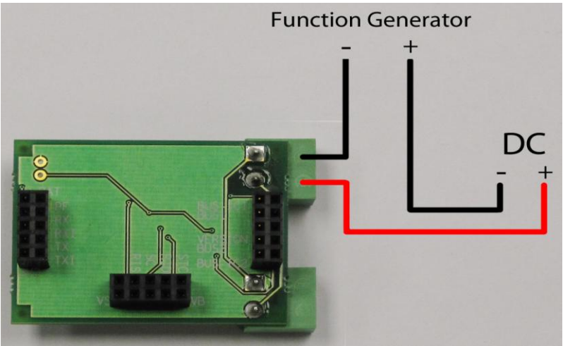
Figure 2: TEST 3 setup
