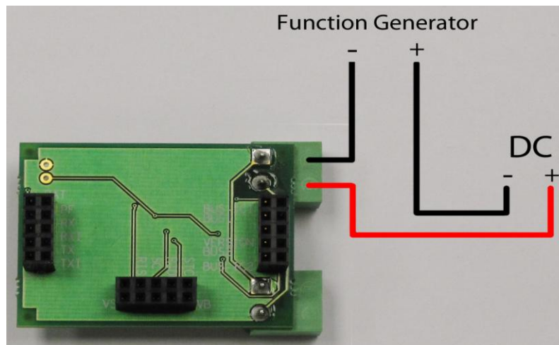
Figure 2: TEST 3 setup
