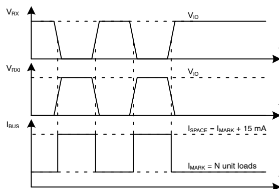
Figure 8. Output Waveforms
