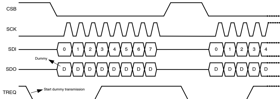
Figure 27. Transmission Request
