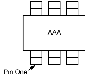
Figure 2. SC70 (Top View)
