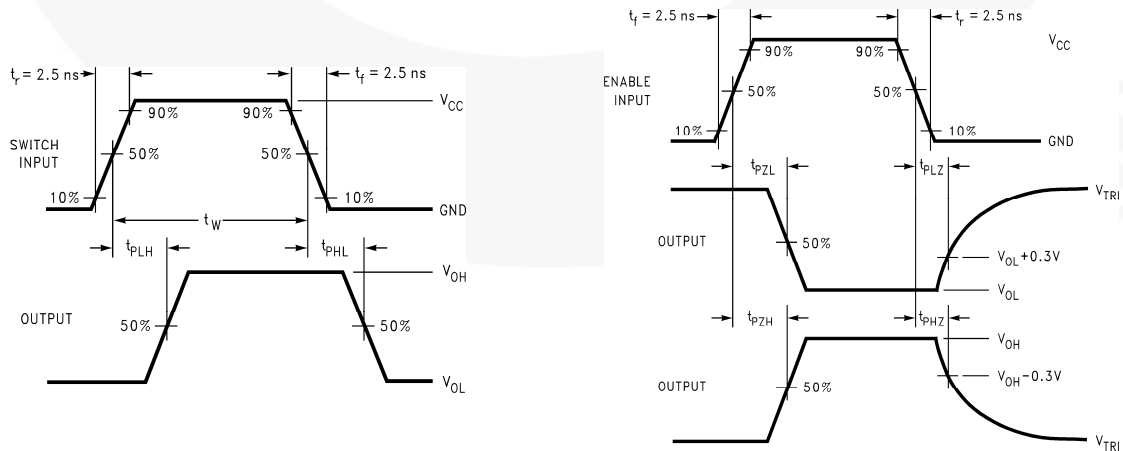
Figure 5. AC Waveforms
