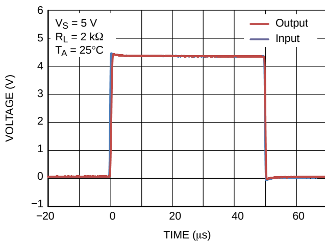
Figure 18. Non-Inverting Large Signal Transient Response
