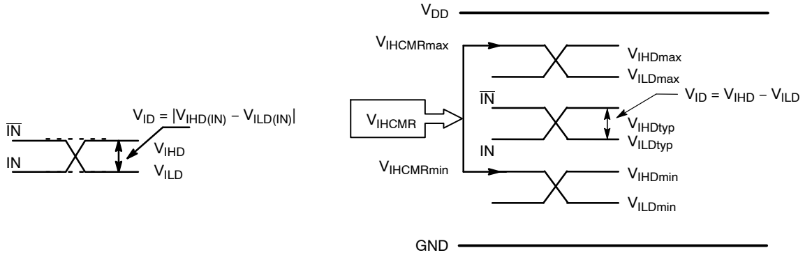
Figure 6. Differential Inputs Driven Differentially
