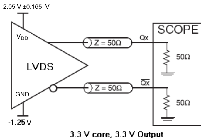
Figure 4. Typical Test Setup and Termination for Evaluation. The V_{DD} of 2.05\text{ V} \pm 0.165\text{ V} and GND of -1.25\text{ V} Split supply allows a direct connection to an oscilloscope 50\ \Omega impedance input module.
