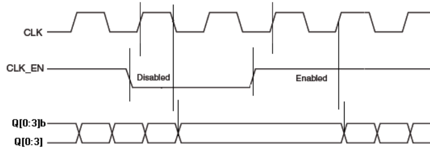
Figure 3. CLK_EN TIMING DIAGRAM
