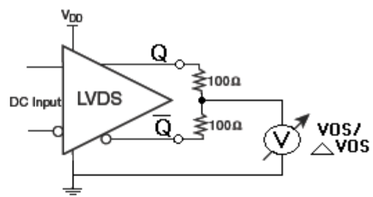
OFFSET VOLTAGE
