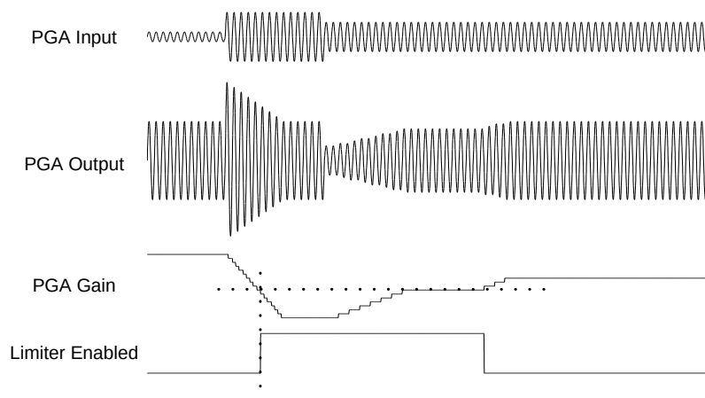
Figure 5: ALC Limiter Mode Operation
