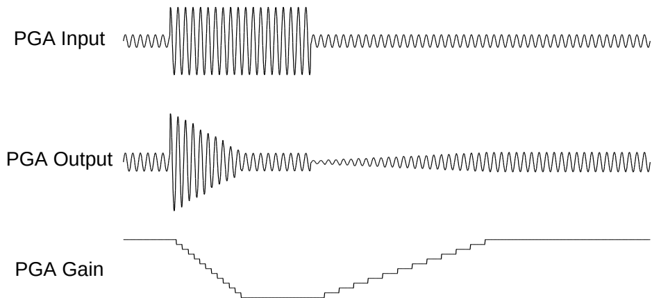
Figure 9: ALC Normal Mode Operation
