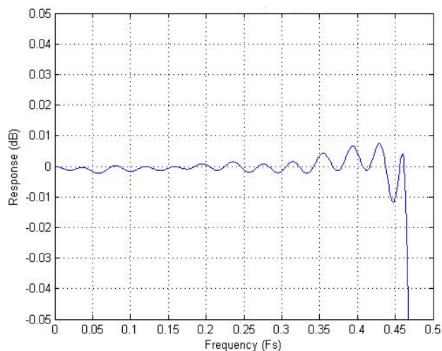
Figure 28: ADC Filter Ripple
