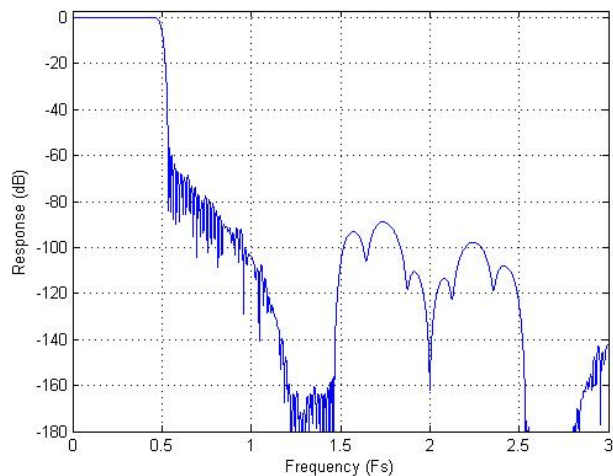
Figure 42: ADC Filter Frequency Response
