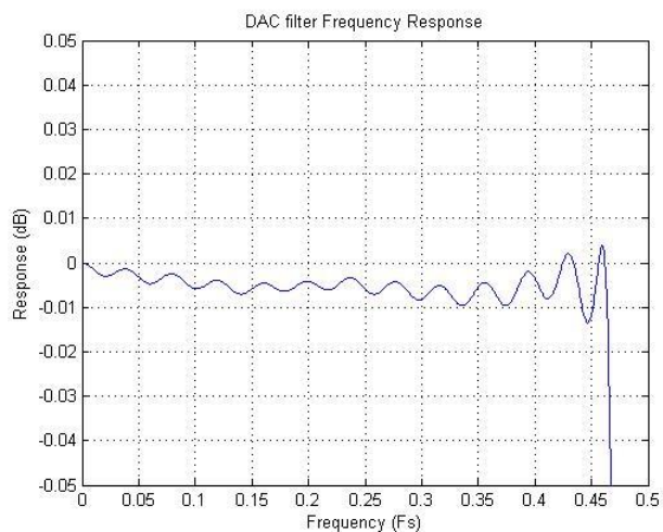
Figure 54: DAC Filter Ripple
