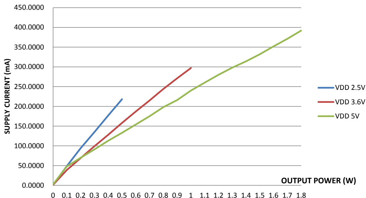
Supply Current vs. Output Power into 8ohm+66uH
