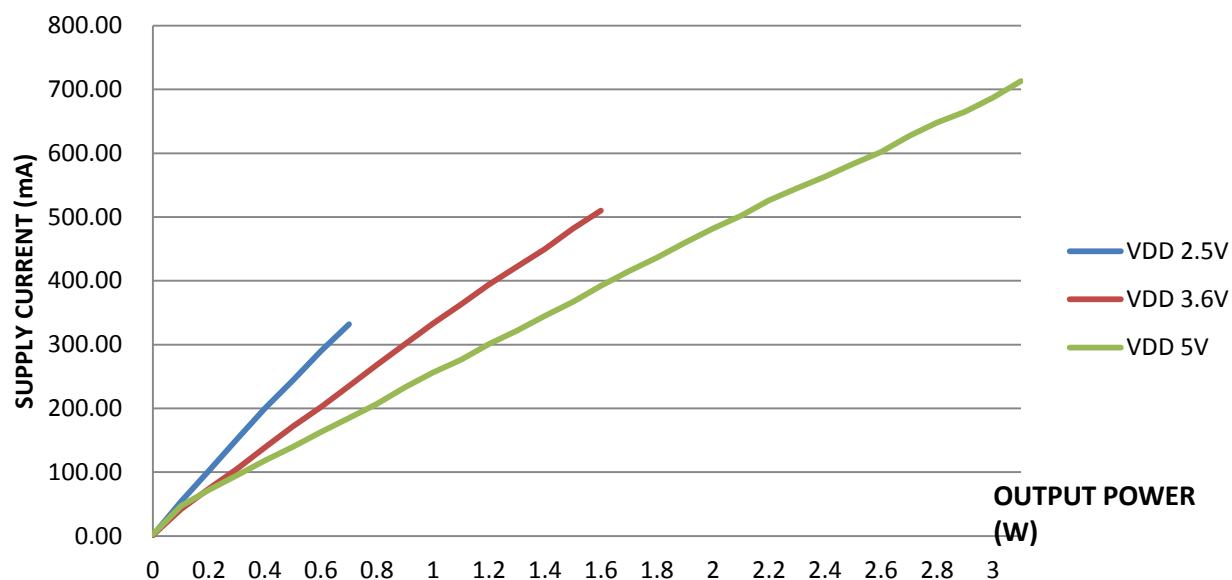
Supply Current vs. Output Power into 4ohm + 33uH
