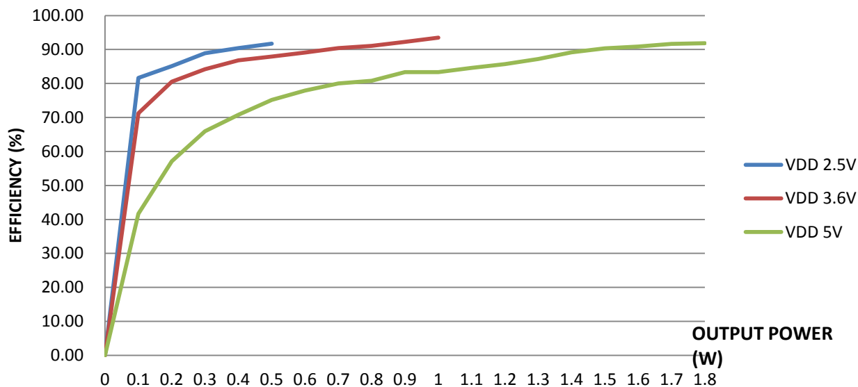
Efficiency vs. Output Power into 8ohm + 66uH
