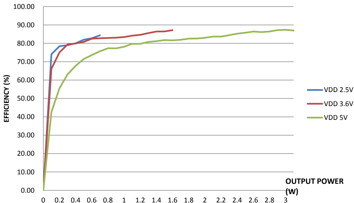
Efficiency vs. Output Power into 4ohm + 33uH
