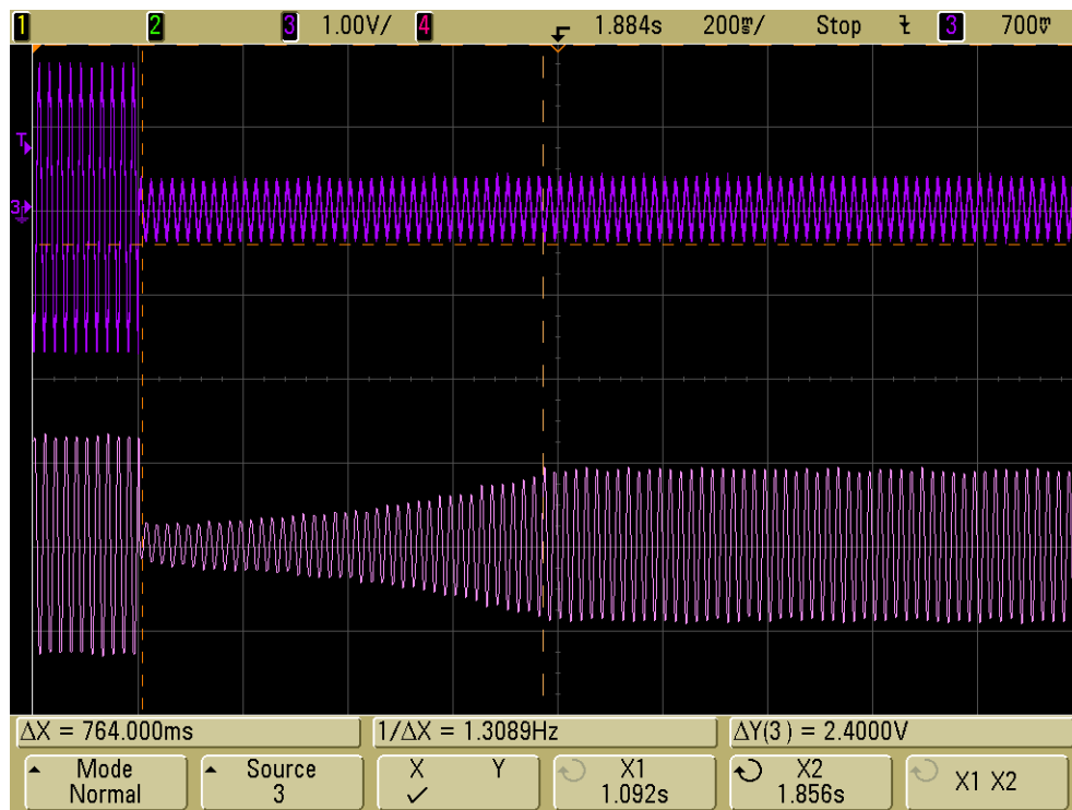
ALC release waveform, VDD 5V Input 0dBV / 3kHz sine Output LC Load 40hm+30uH
