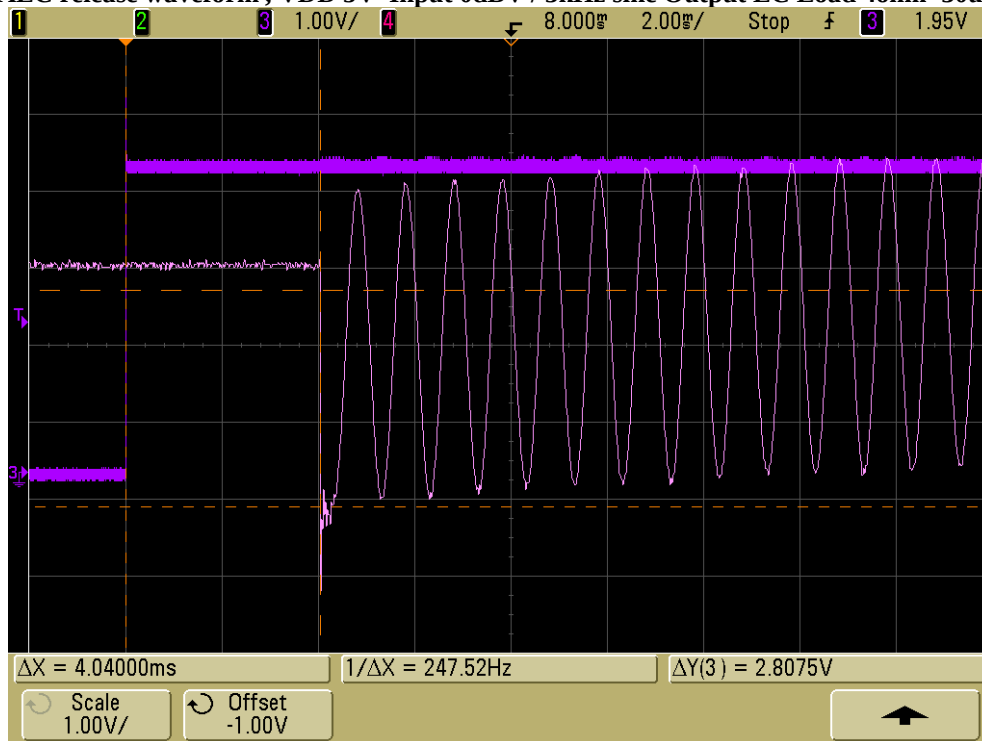
Start up time 4ms, VDD 5V Input 0dBV / 1kHz sine Output LC Load 40hm+30uH
