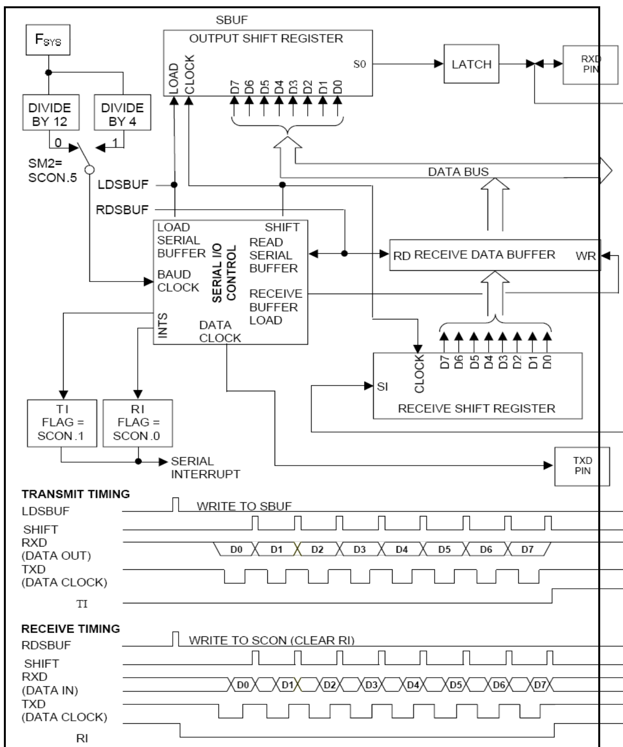
Figure 12-1 Serial Port Mode 0 Function Block
