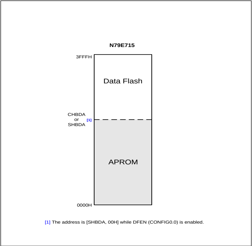
Figure 6-2 N79E715 Data Flash
