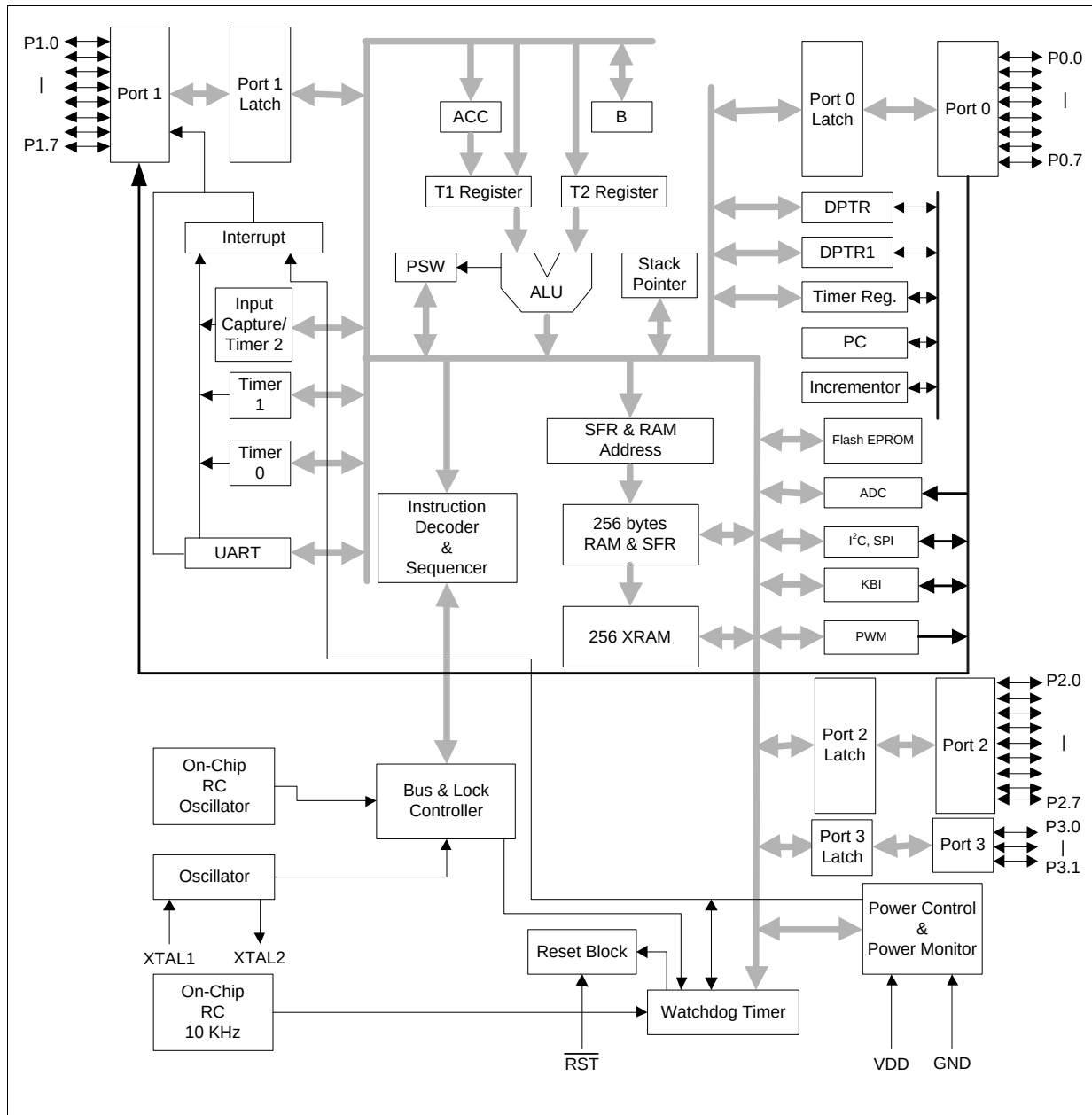
Figure 4-1 N79E715 Function Block Diagram
