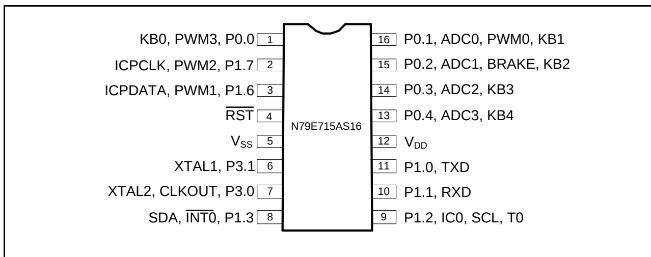
Figure 5-5 SOP 16-pin Assignment
