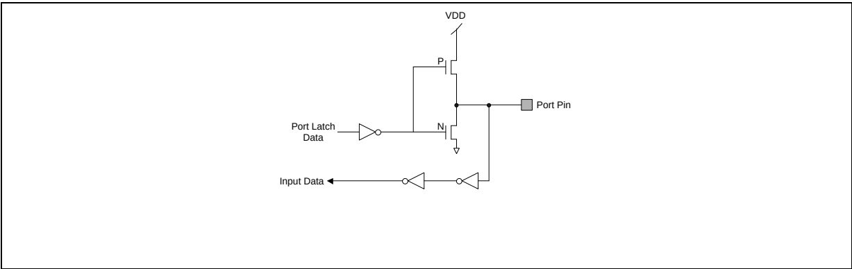
Figure 9-3 Push-Pull Output
