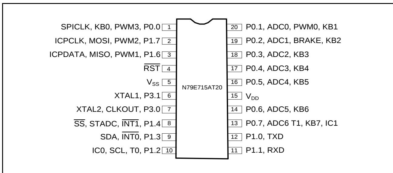
Figure 5-2 TSSOP 20-pin Assignment
