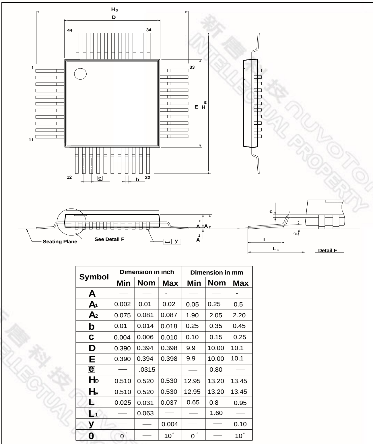
Figure 27-3. PQFP-44 Package Dimention
