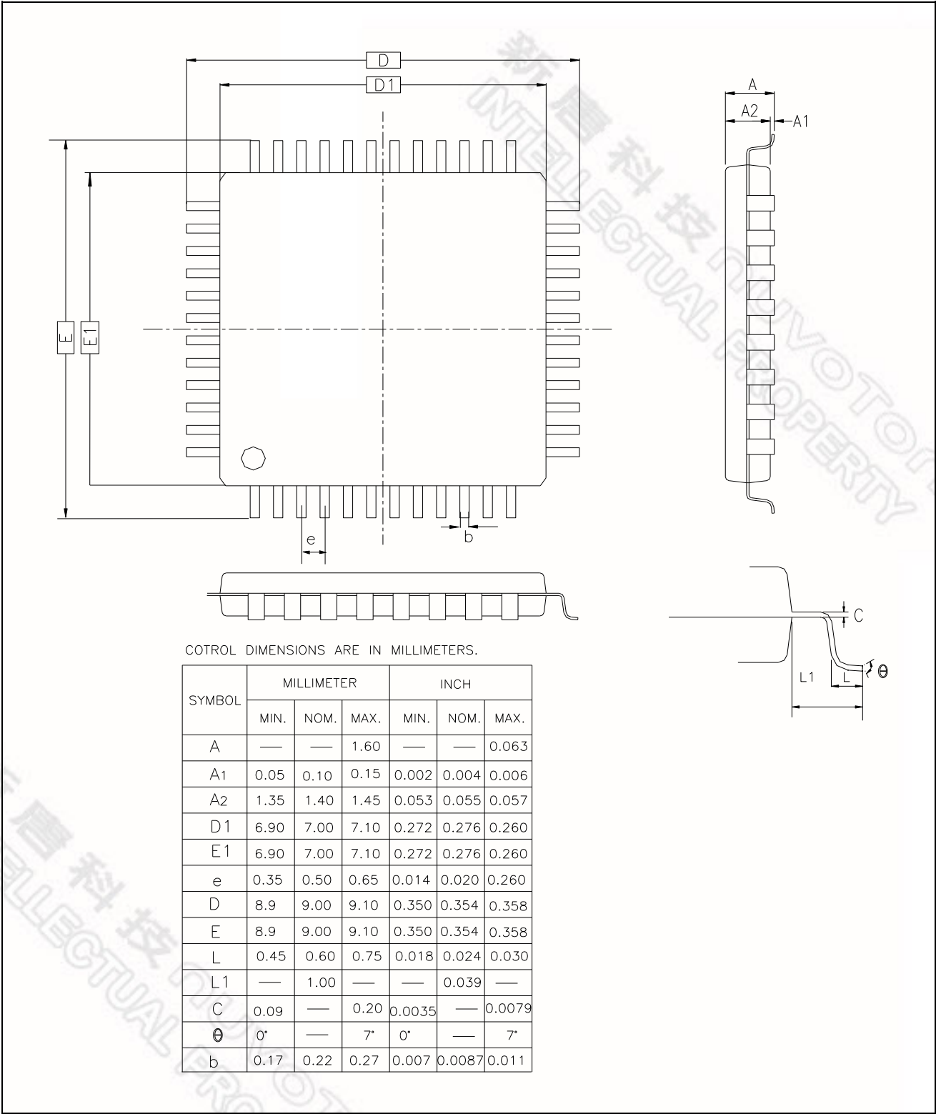
Figure 27-5. LQFP-48 Package Dimention
