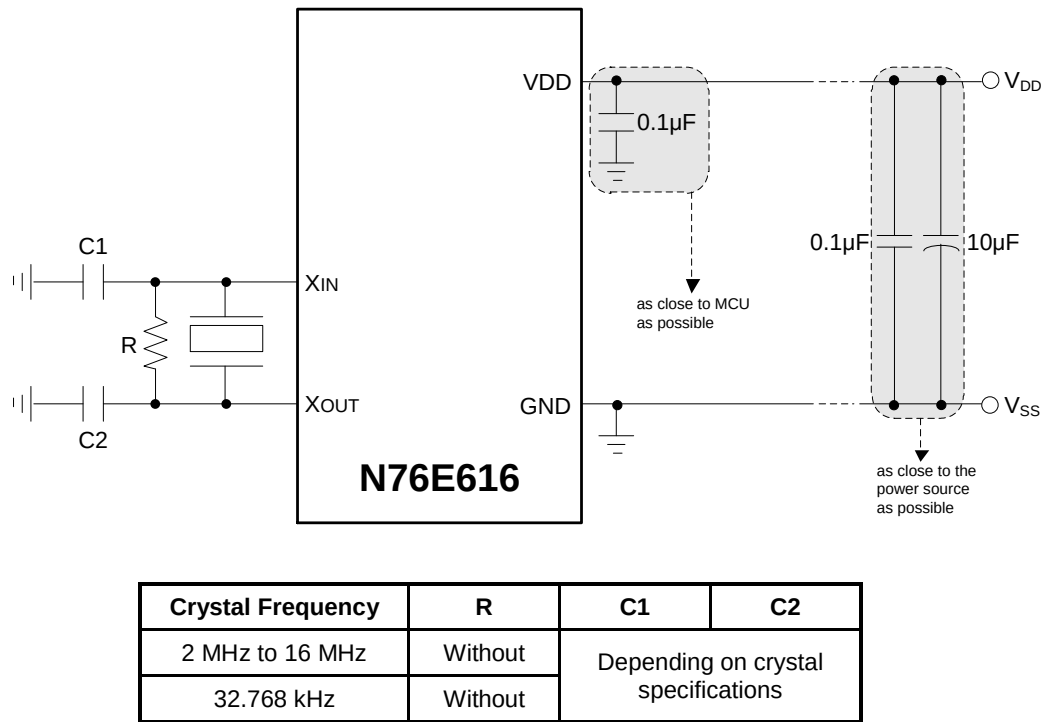
Figure 4.4. Application Circuit with External Crystal
