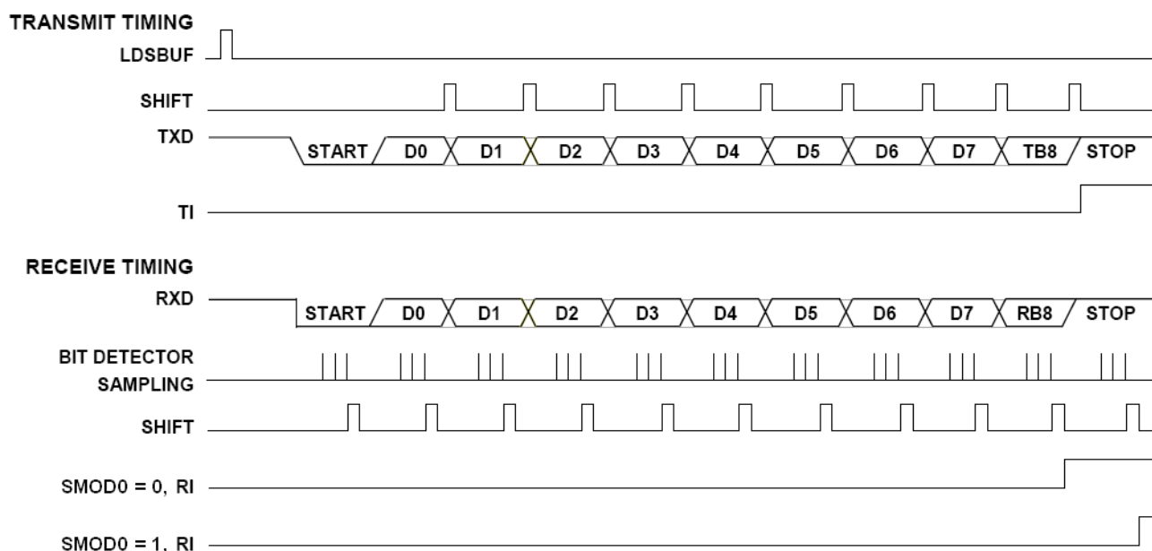
Figure 14.3. Serial Port Mode 2 and 3 Timing Diagram
