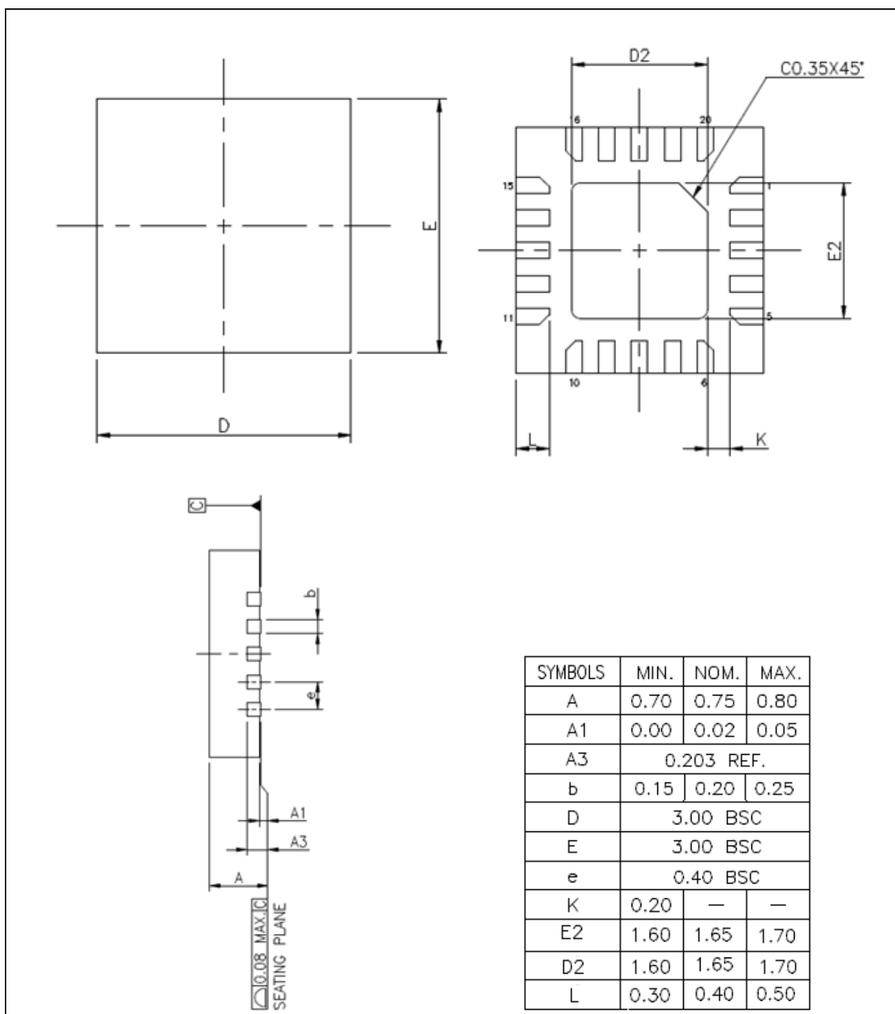
Figure 32.3. QFN-20 Package Dimension of N76E003AQ20
