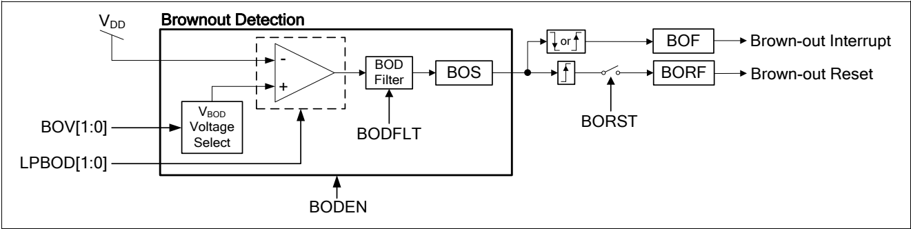
Figure 24.1. Brown-out Detection Block Diagram
