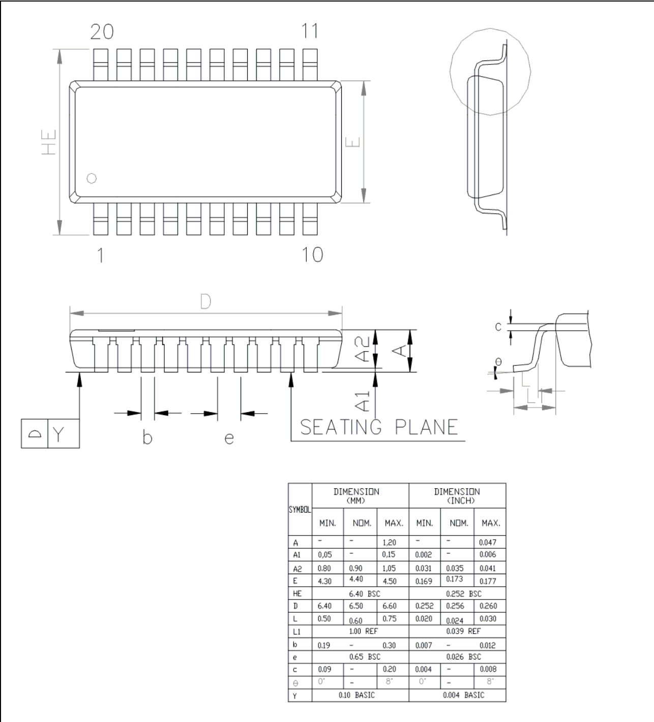
Figure 32.1. TSSOP-20 Package Dimension
