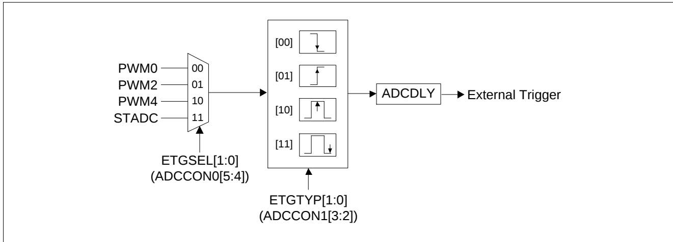
Figure 18.2. External Triggering ADC Circuit
