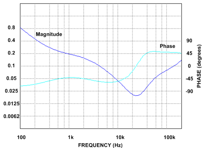
Model N6753A and N6755A, Option 760, CC Mode, @20 V, 15A
