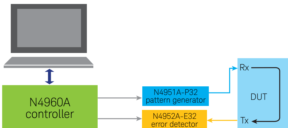
Figure 20. Test setup for communication ICs.
