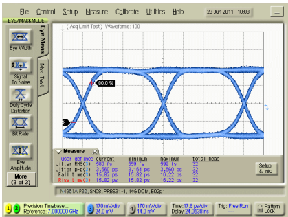
Figure 2. Typical eye at 14 Gb/s.
