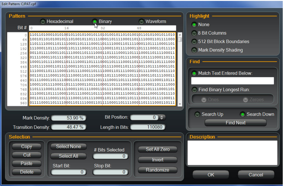
Figure 13. Sub-pattern editor.
