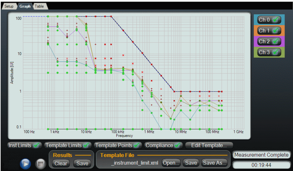
Figure 16. Jitter tolerance graph view.
