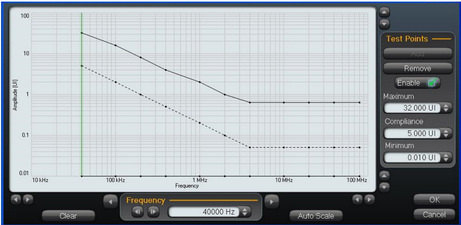
Figure 18. Template file.
