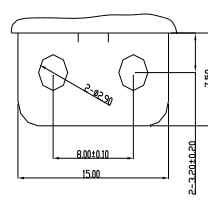
DETAIL D SCALE 5:1
