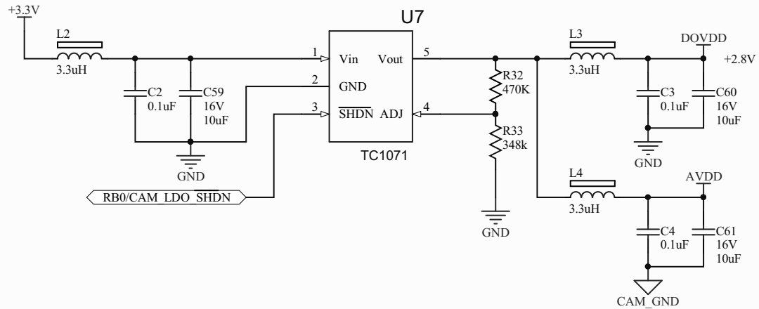
FIGURE A-9: VGA CAMERA SENSOR AND 2.8V REGULATOR
