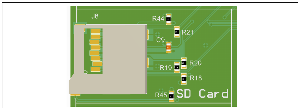
FIGURE 2-11: microSD CARD SLOT
