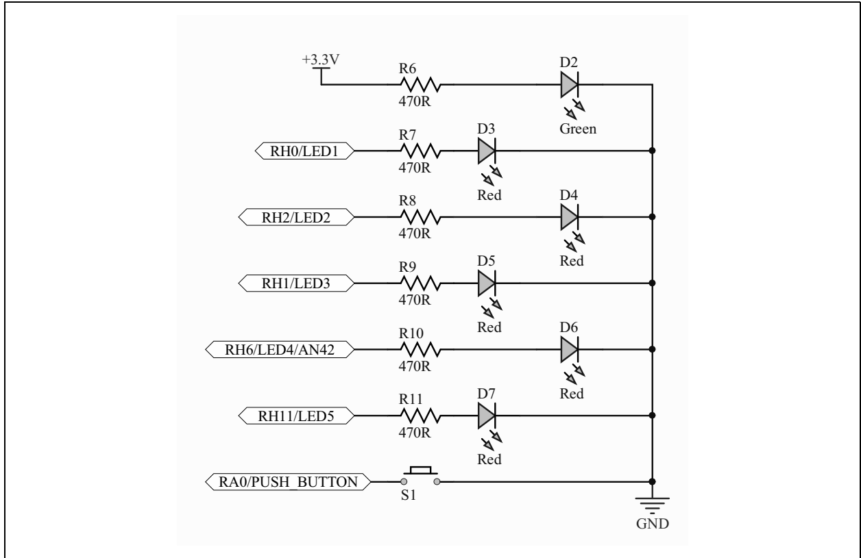
FIGURE A-18: PUSH BUTTON AND USER CONTROLLED LEDS
