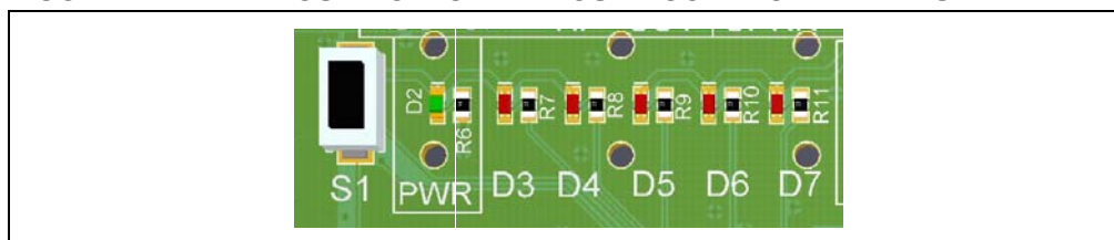
FIGURE 2-14: PUSH BUTTON AND USER CONTROLLED LEDs
