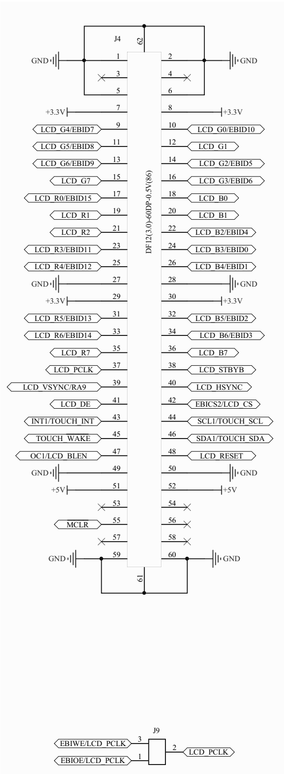
FIGURE A-7: DISPLAY CONNECTOR
