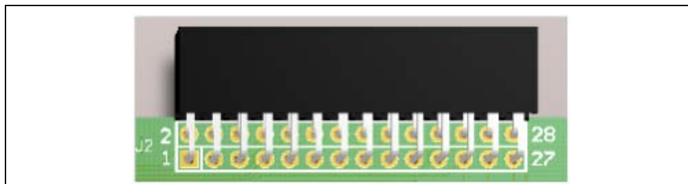
FIGURE 2-13: PICtail™ CONNECTOR
