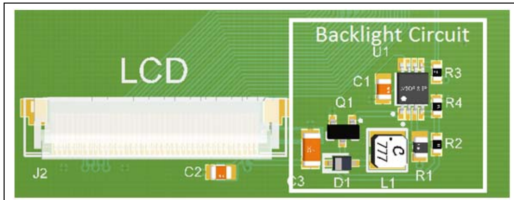
FIGURE 2-15: DISPLAY PANEL CONNECTOR AND BACKLIGHT CIRCUIT
