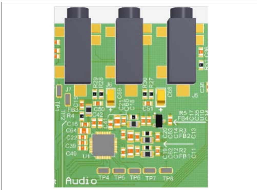
FIGURE 2-6: 24-BIT AUDIO CODEC
