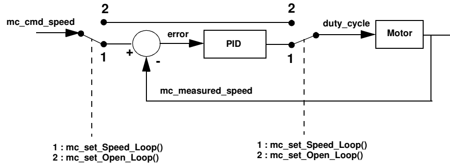
Figure 9. Regulation Loop
