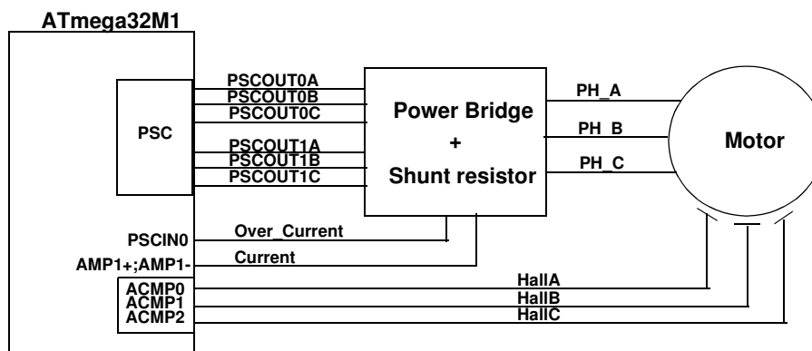
Figure 6. Hardware implementation
