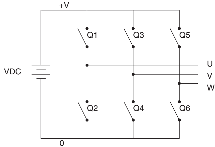
Figure 4. Power Stage
