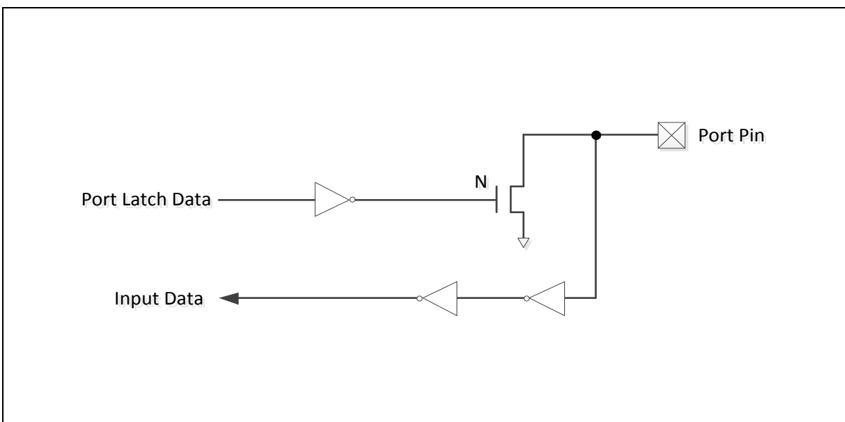
Figure 6.5-4 Open-Drain Output
