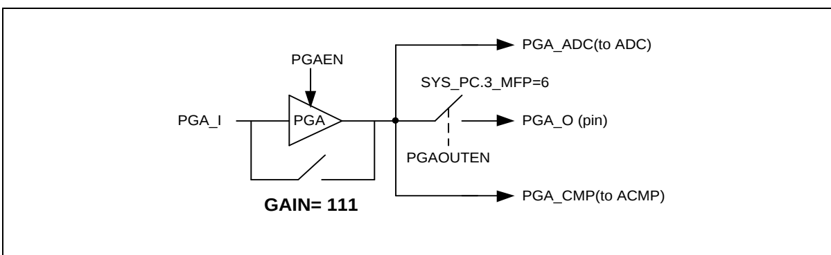
Figure 6.18-1 OP Amplifier Block Diagram
