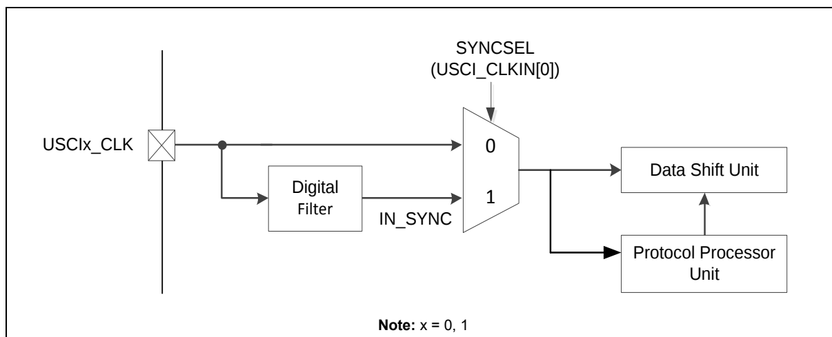
Figure 6.11-3 Input Conditioning for USC1x_CLK
