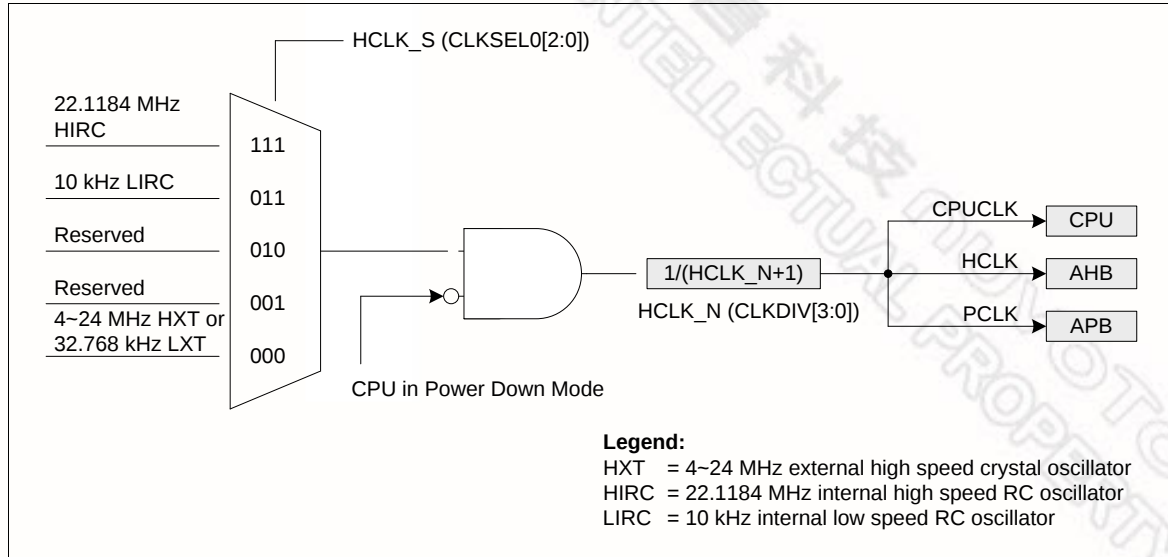
Figure 6.4-2 System Clock Block Diagram
