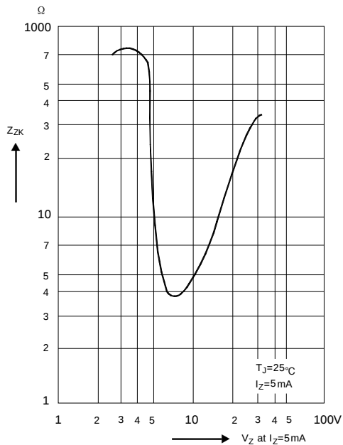
Dynamic resistance versus Zener voltage
