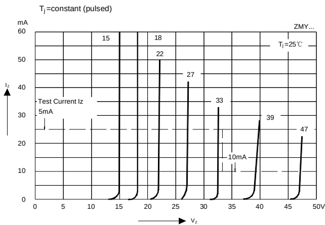
FIG.3-BREAKDOWN CHARACTERISTICS
