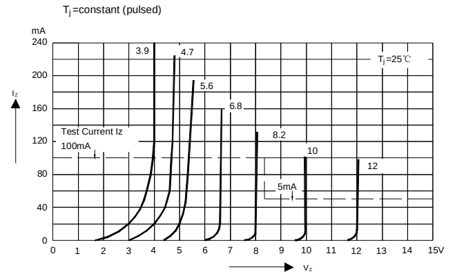
FIG.2-BREAKDOWN CHARACTERISTICS
