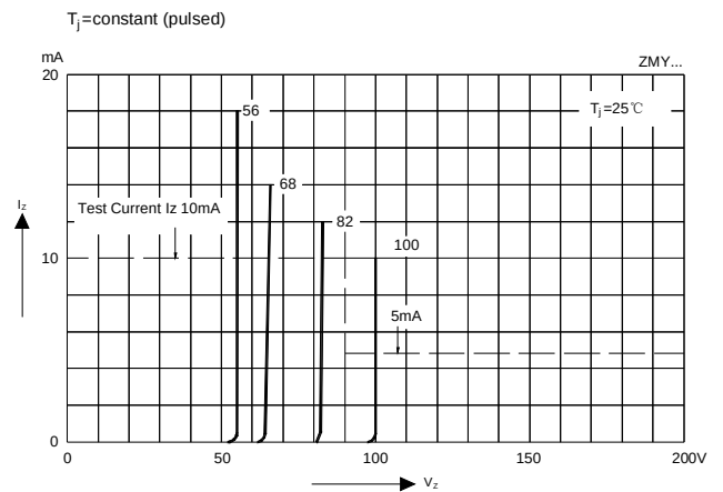
FIG.4-BREAKDOWN CHARACTERISTICS
