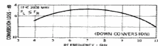
Conversion Loss vs. Frequency
