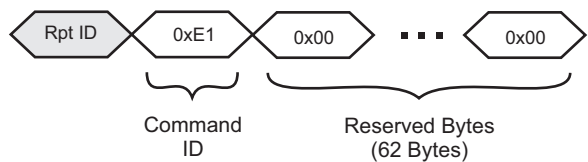
FIGURE 10-16: START DEBUG MONITORING – RESPONSE PACKET FORMAT
