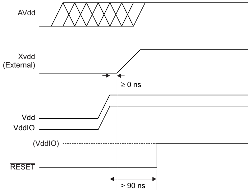
FIGURE 5-1: POWER SEQUENCING ON THE MXT1664T3
