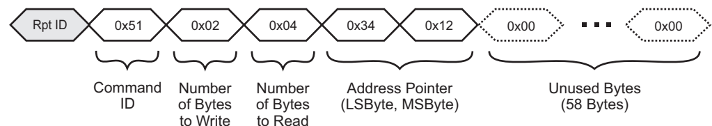
FIGURE 10-7: EXAMPLE OF A FOUR-BYTE READ STARTING AT ADDRESS 0x1234
