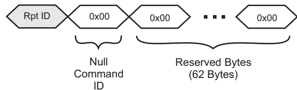
FIGURE 10-13: SEND AUTO-RETURN – NULL COMMAND PACKET FORMAT
