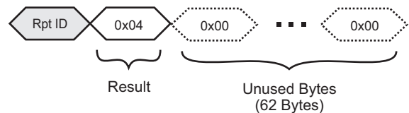
FIGURE 10-6: RESPONSE TO EXAMPLE FOUR-BYTE WRITE
