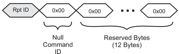
FIGURE 9-12: SEND AUTO-RETURN – NULL COMMAND PACKET FORMAT
