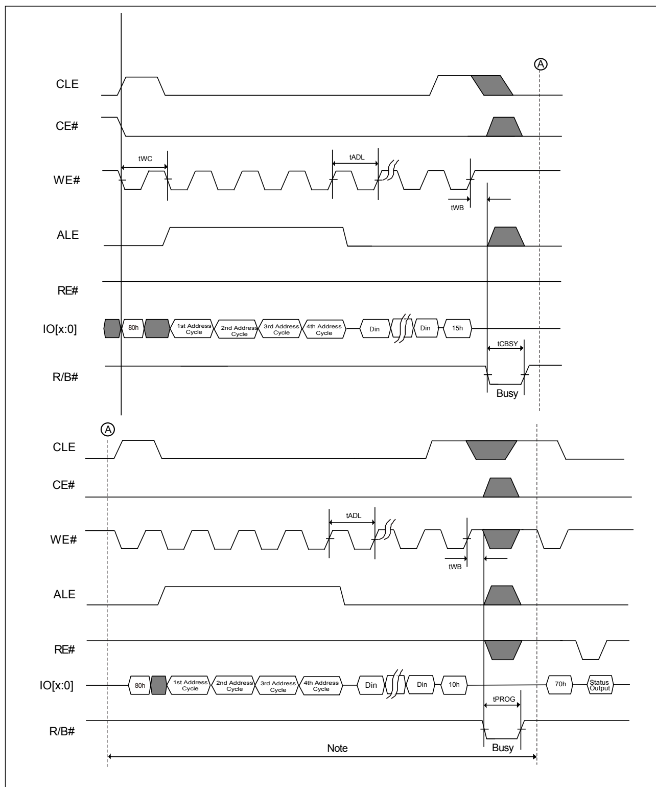
Figure 15-1. AC Waveforms for Cache Program
