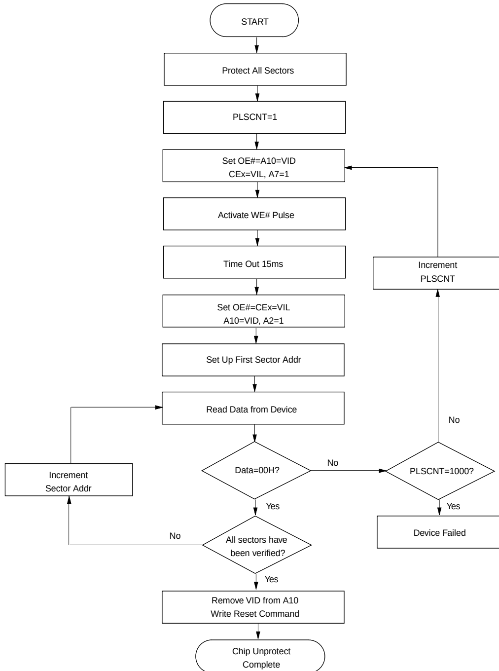
Figure 19. CHIP UNPROTECT FLOWCHART (A10, OE# Control)
