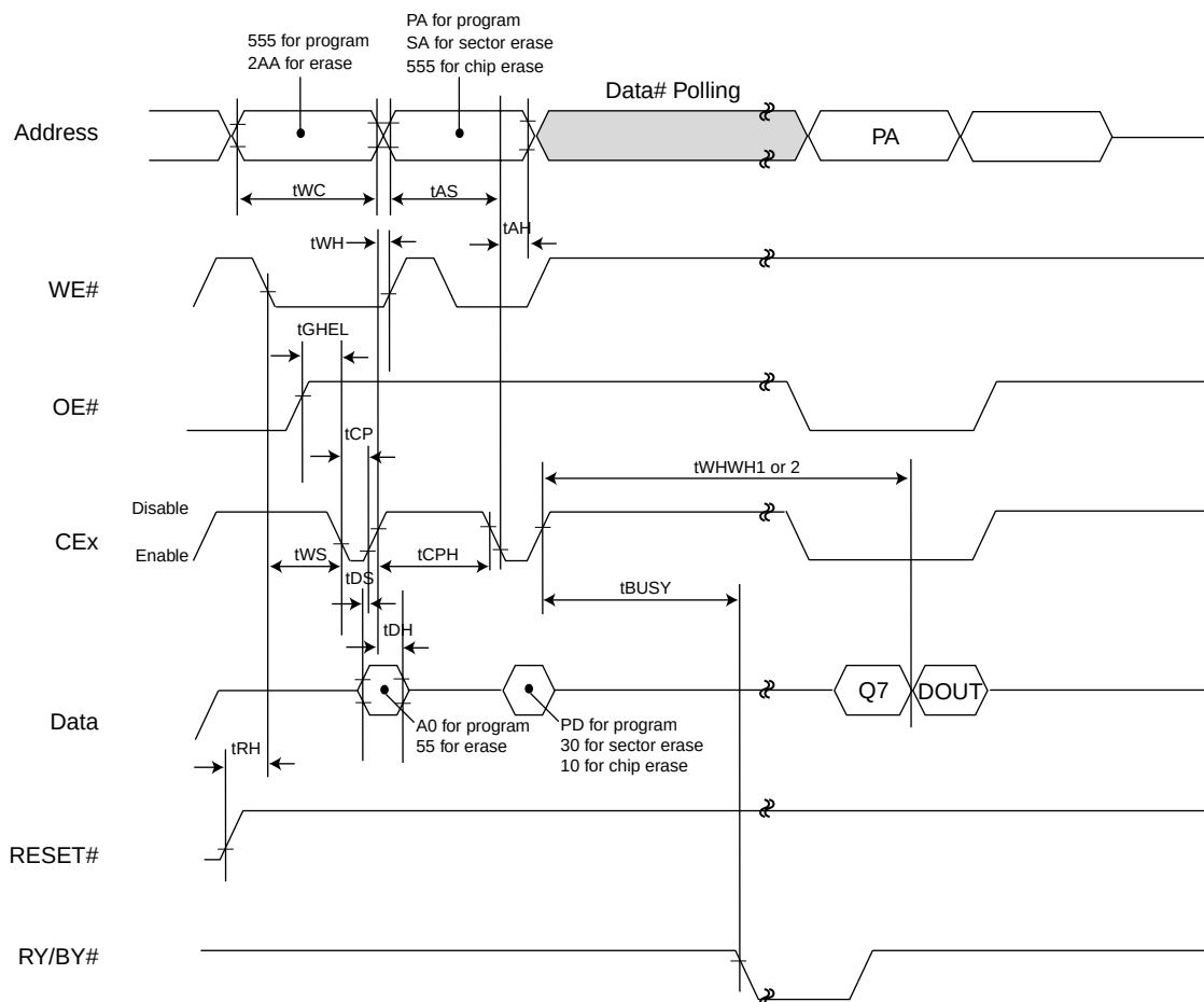
Figure 13. CEx CONTROLLED PROGRAM TIMING WAVEFORM
