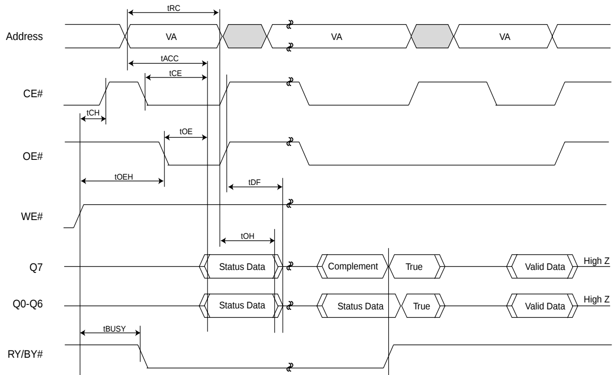
Figure 24. DATA# POLLING TIMING WAVEFORMS (DURING AUTOMATIC ALGORITHMS)
